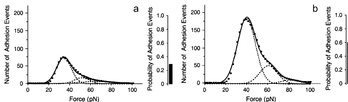
FIGURE 7 Analysis of force distributions of aortic EC before (a) and after (b) histamine treatment performed by simultaneous deconvolution of the experimental data (■) with Gaussian distributions to resolve the integrin-fibronectin binding forces. Although histamine treatment preserved the overall shape of the force distribution, it increased adhesion probability and shifted the entire force distribution toward higher force values. The histogram bar shows the probability of adhesion events.
