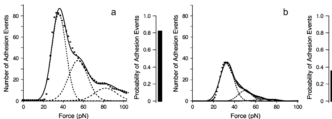
FIGURE 11 Analysis of force distributions for the GRGESP/GRGDdSP experiment. The GRGESP control force distributions (a) and the treatment GRGDdSP (b) are preserving the same overall shape, but GRGDdSP treatment recorded an important decrease in adhesion events. None of these peptides affected the magnitude of the adhesion force between fibronectin and \alpha 5 \beta 1 integrin.
